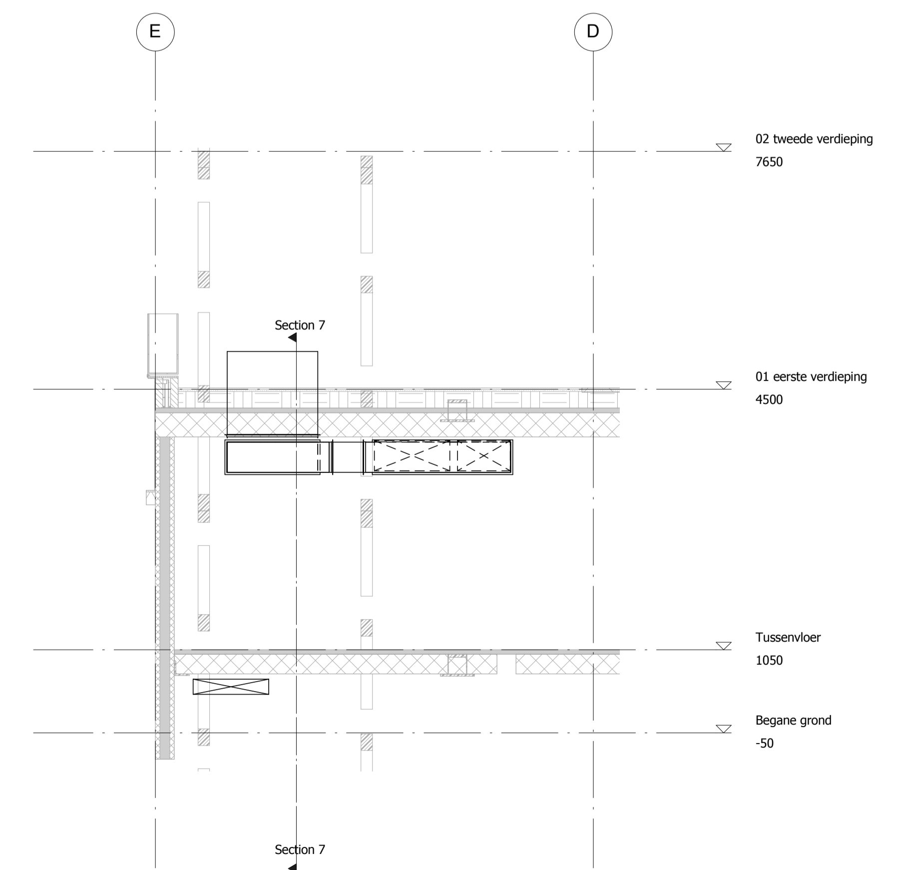
2 Wand op as 7 1:50
