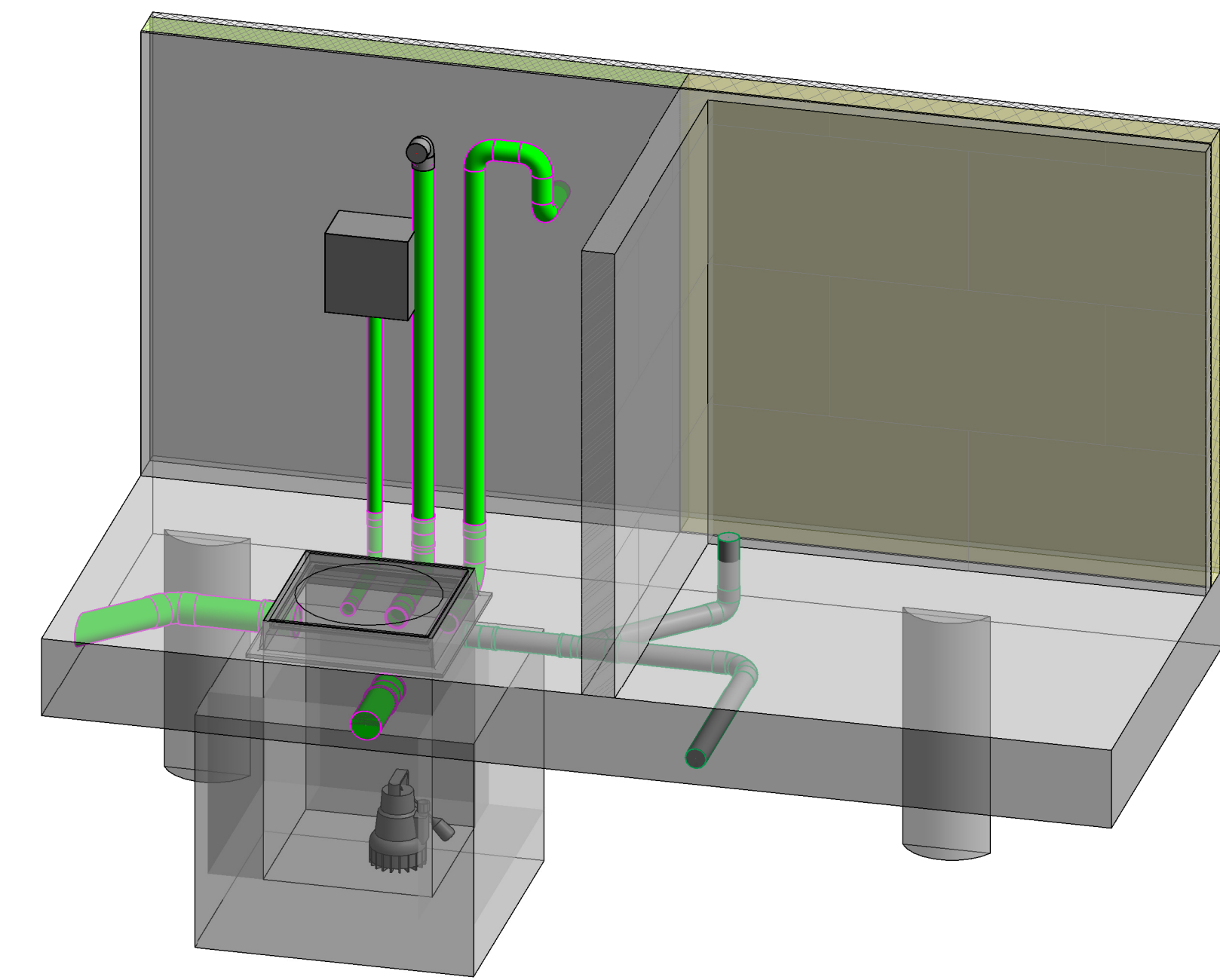
6 pompput 3d - plot
